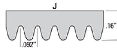
J cross-section from 13" to 98"
