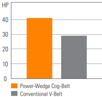
5V Section Drive, 750 RPM, 1.5:1 Belt Drive Ratio
